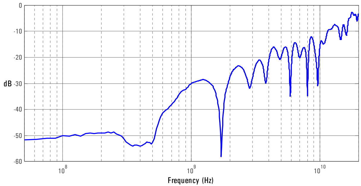
Magnitude plot of differential return loss.
